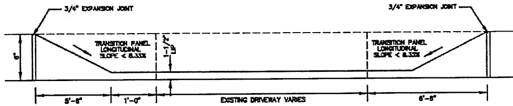
CURB LINE PROFILE
