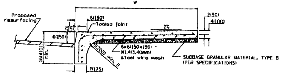
COMBINATION CURB - SIDEWALK 4" (100mm) Measurement Formula: W \times \text{length constructed} = \text{Payment area} in square meters/square feet
