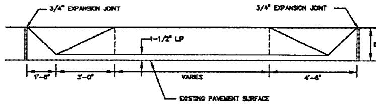
CURB LINE PROFILE
